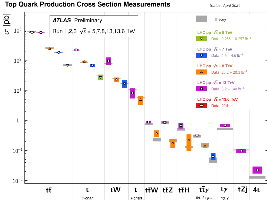
Figure 2.2.: Overview of several t quark related production cross-section measurements with theoretical predictions calculated at next to leading order or higher [48].
