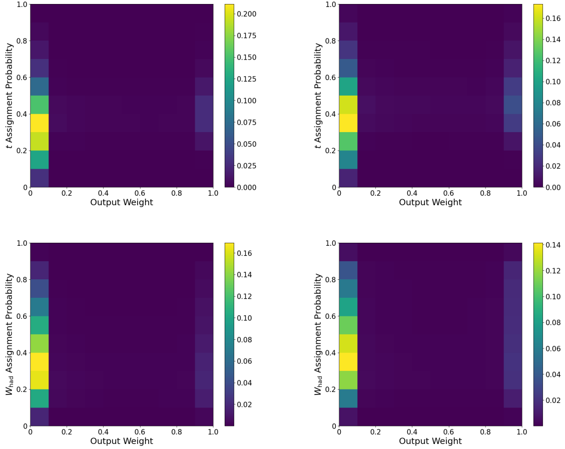
Figure 7.5.: Histogram combining SPA-Net 's assignment probability and Neutrino Weighting outputs for (left) background events and (right) signal events. here the partons are split into (upper) t quark and (lower) W_{\text{had}} from H -boson decay. The signal events have higher contributions in upper probability and weight regions.
