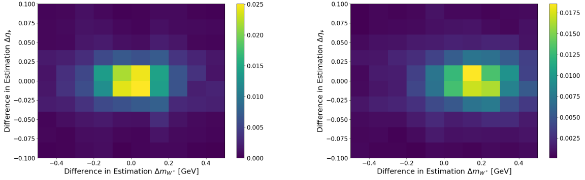
Figure 8.3.: Comparison of two heatmaps showing the difference between the estimated and true values. The two heatmaps use (left) the correct m_H = m_H^{\text{MC}} and (right) the off-set m_H = 125.20 \text{ GeV} .
