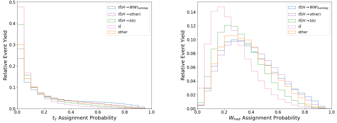
Figure 7.3.: Distributions of different event topologies for SPA-Net 's assignment probabilities of (left) the top t_2 and (right) the hadronic W -boson from the Higgs decay.
