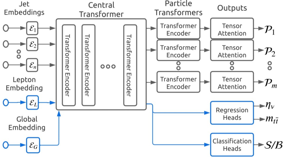
Figure 5.1.: Overview of SPA-Net 's architecture including its four regions and the additional embeddings for additional lepton and global information such as the missing transverse energy [68].
